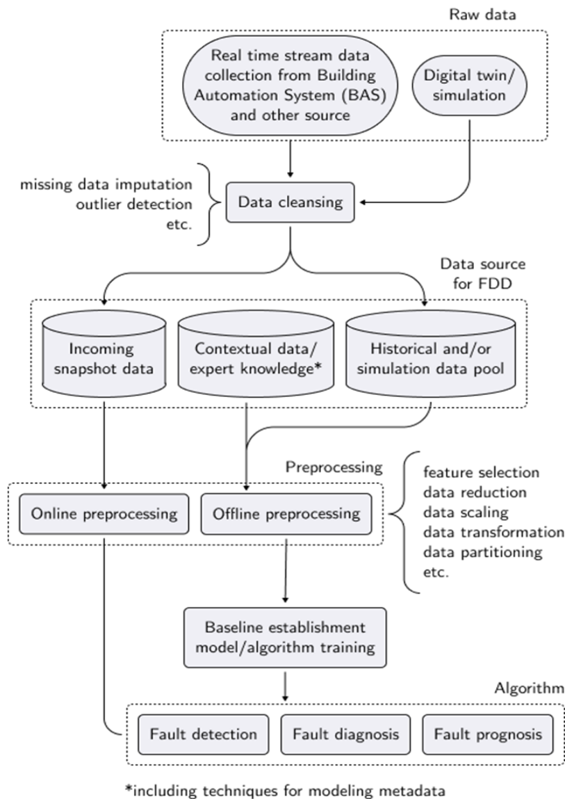
Figure 5 A General Data-driven FDD Process.
