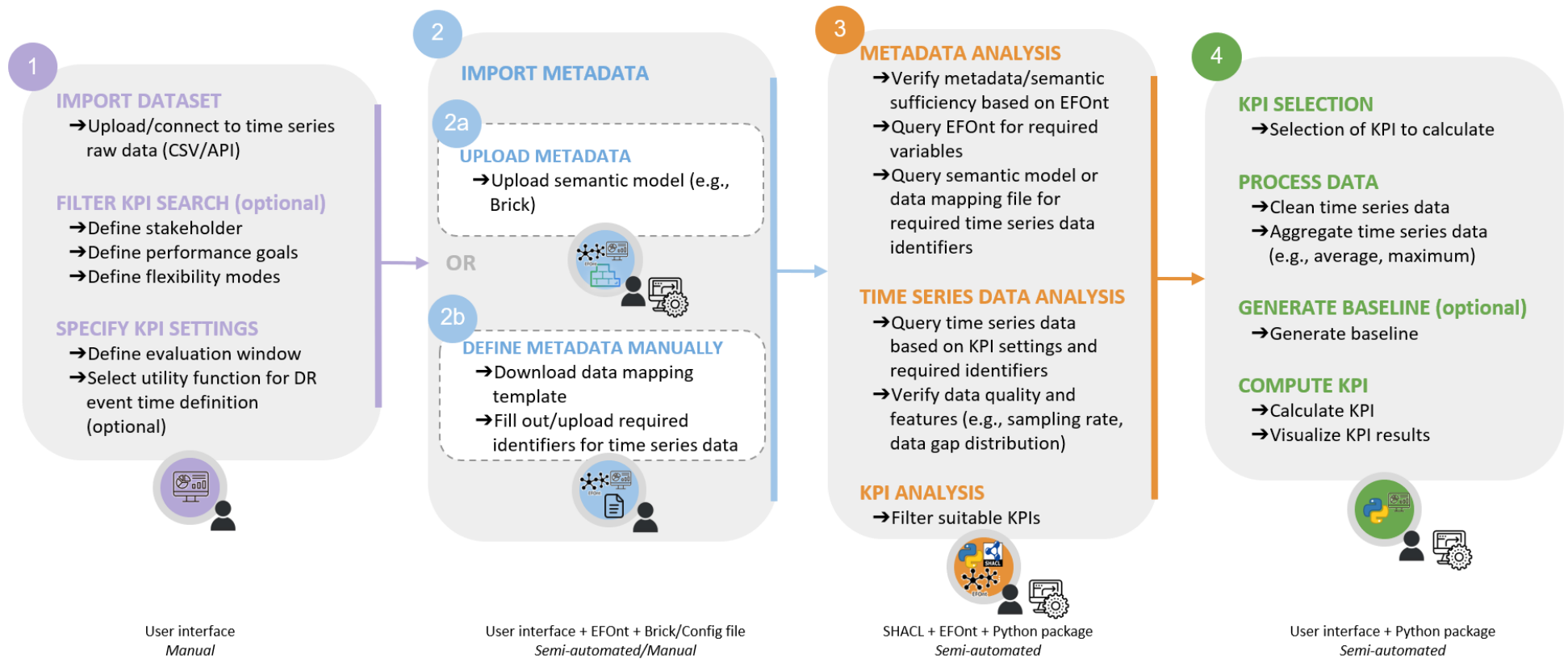
Figure 11 Data-driven energy flexibility quantification process for B2G applications [51].
